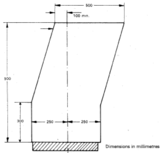
Fig. 3 Zone of clearance
