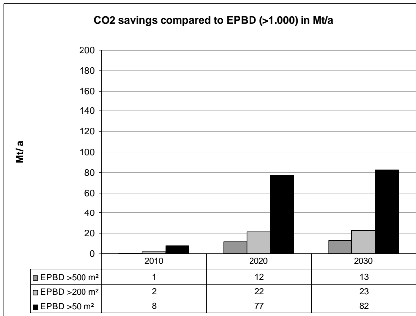
Figure 2.7 CO 2 savings compared to current EPBD from different threshold options
