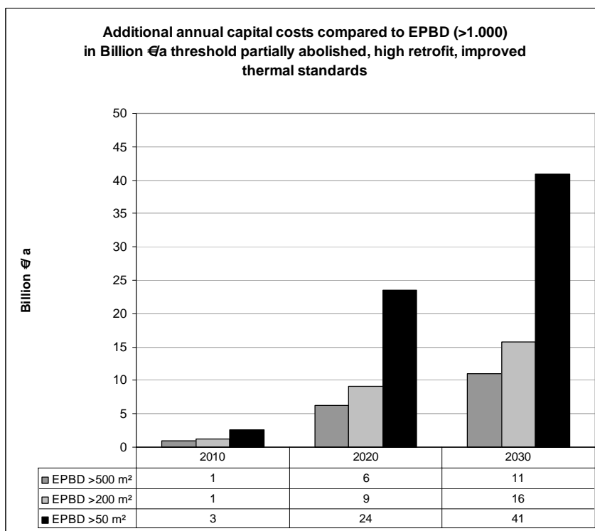
Figure 2.26 Additional annual capital costs compared to current EPBD (>1.000) in Billion €a threshold already partially abolished, high retrofit, improved thermal standards
