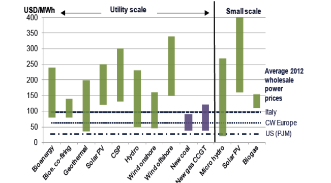
Figure 18: Levelised costs of power generation (USD per megawatt hour), first quarter 2013
