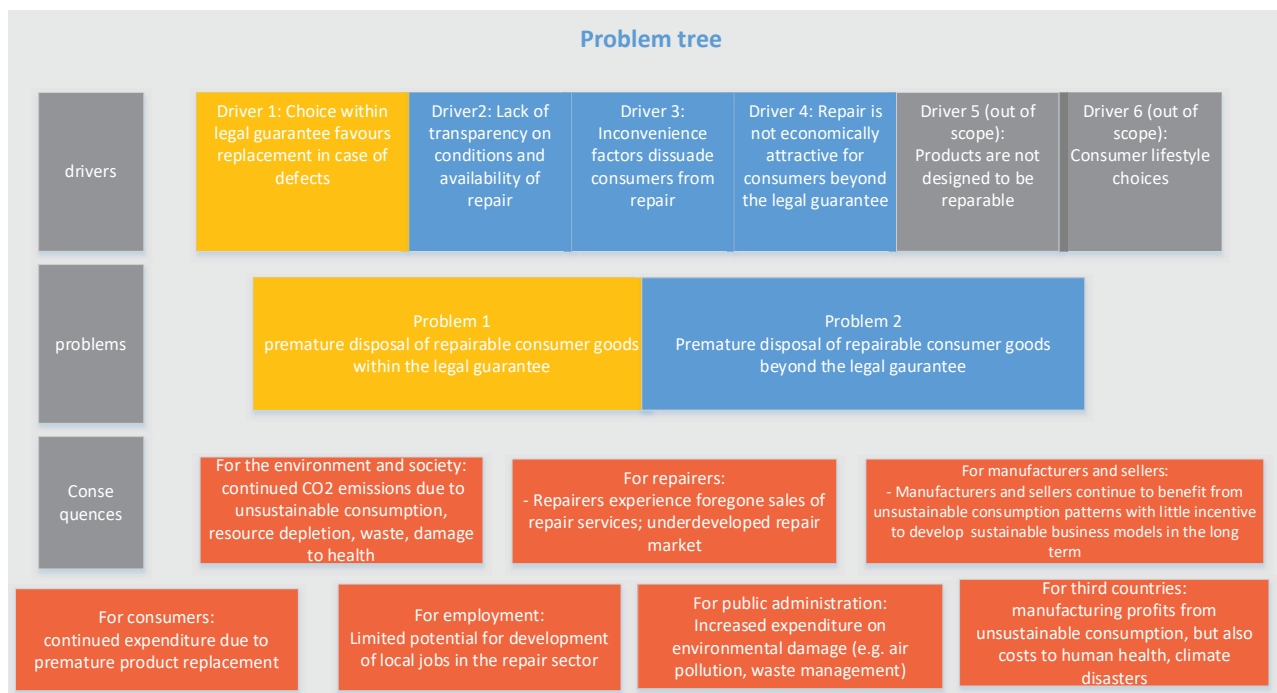
Figure 1: Problem tree
